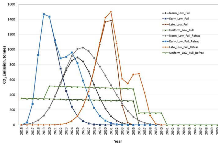
Fig. 7. Annual CO 2 emissions for all timelines, under low well development, assuming full fracking water demand met by tanker, with and without re-fracturing.
