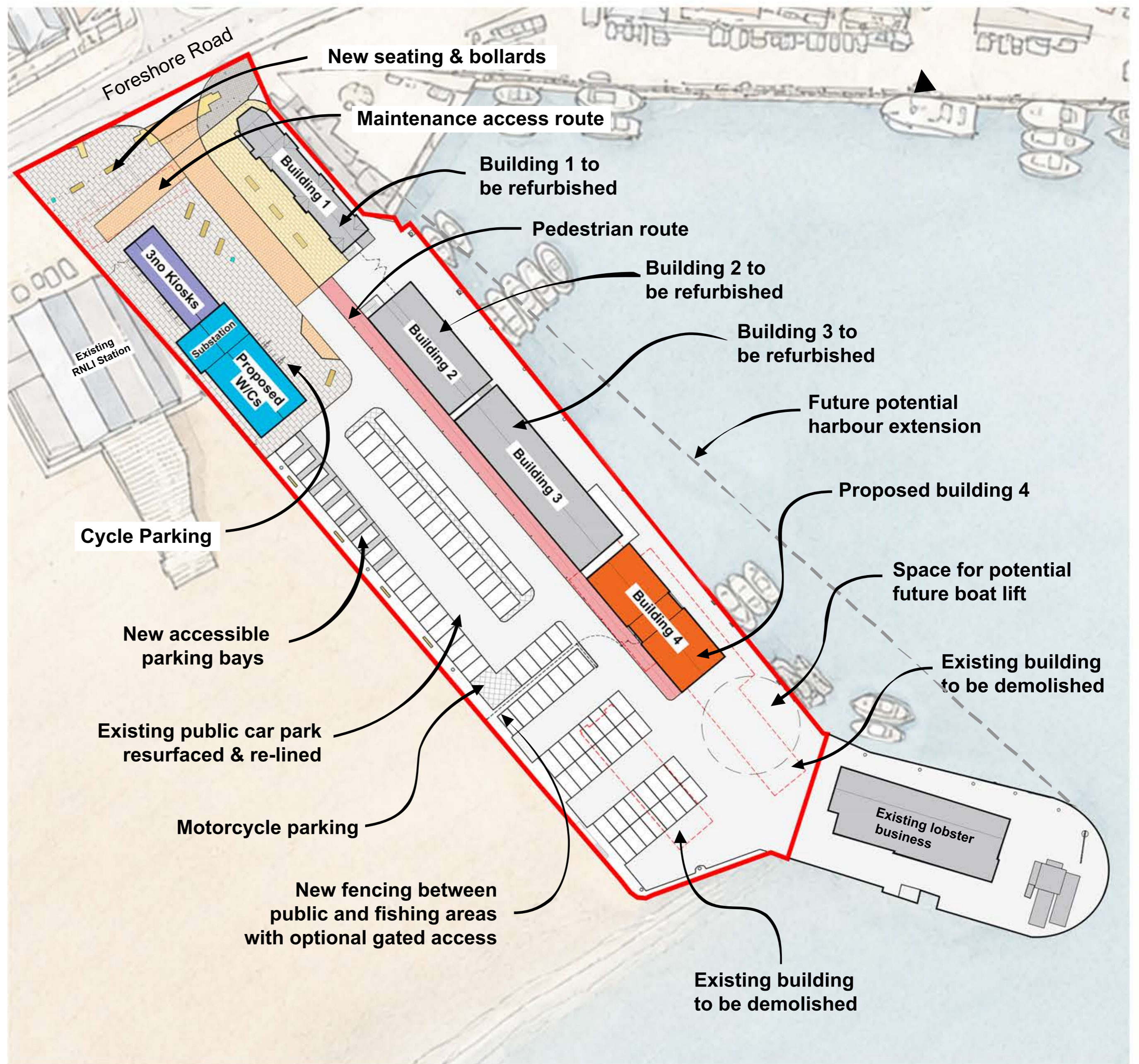
Indicative Proposed Site Plan.
