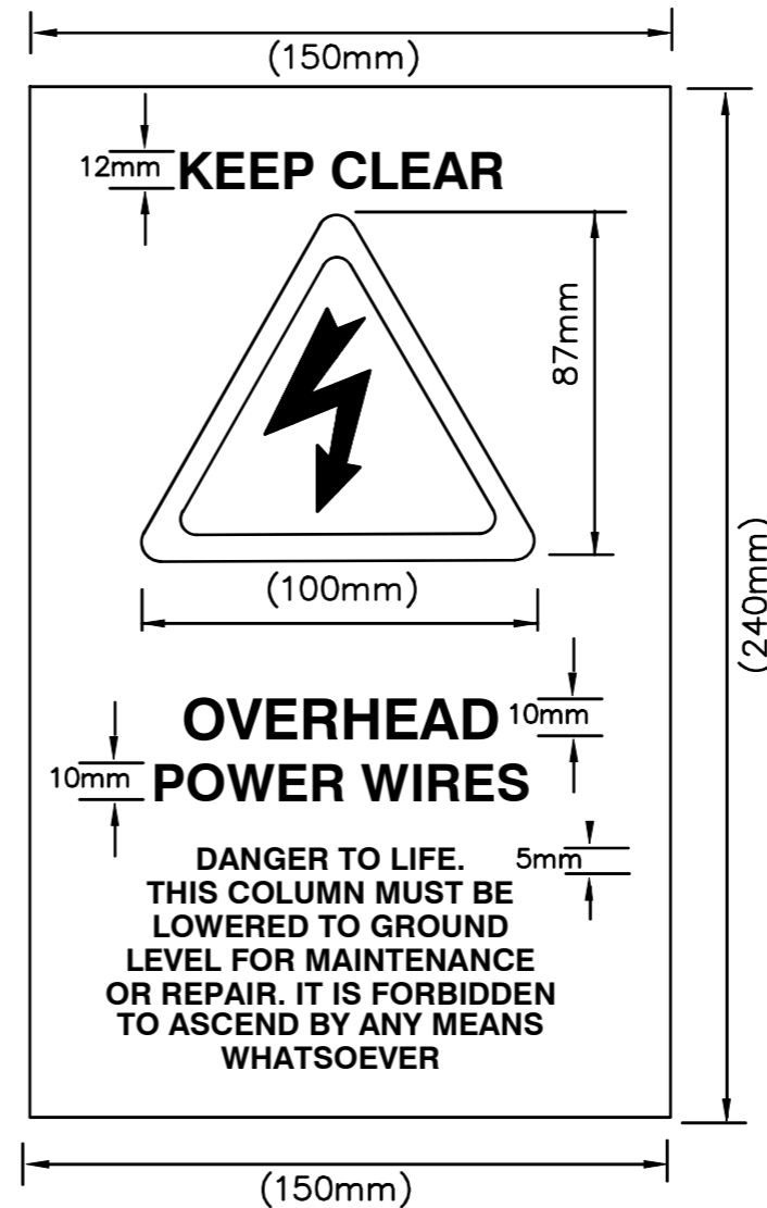
TYPE II TO BE FIXED AT BOTTOM OF COLUMN SHAFT
