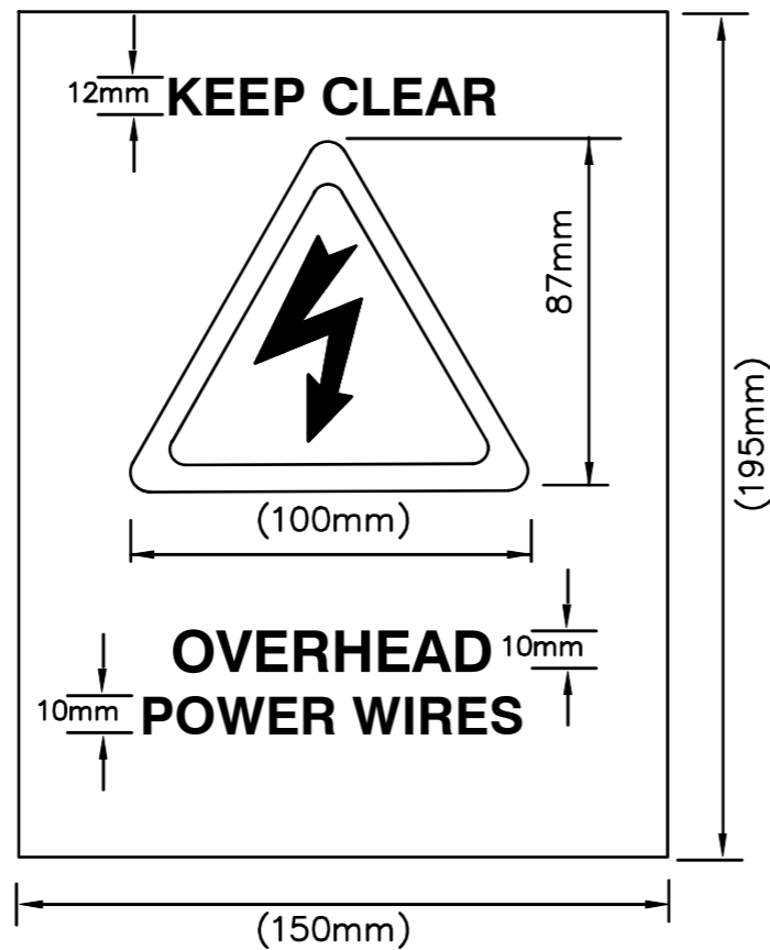
TYPE I TO BE FIXED AT TOP AND BOTTOM OF COLUMN
