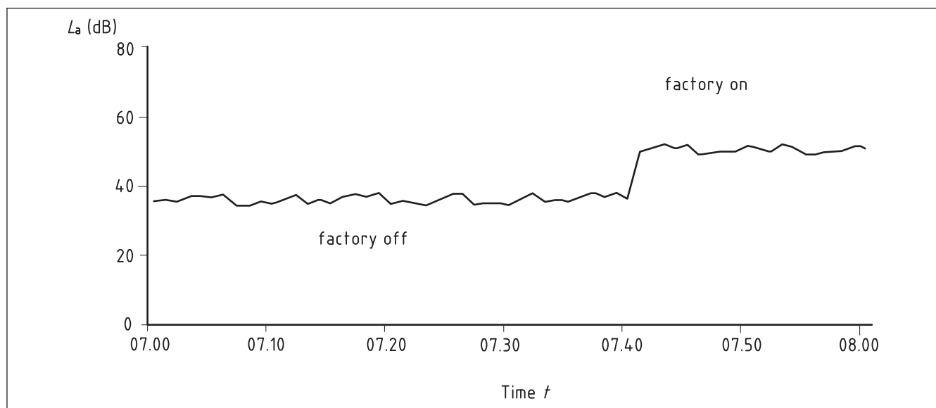
Figure A.1 Sound level variation with time
