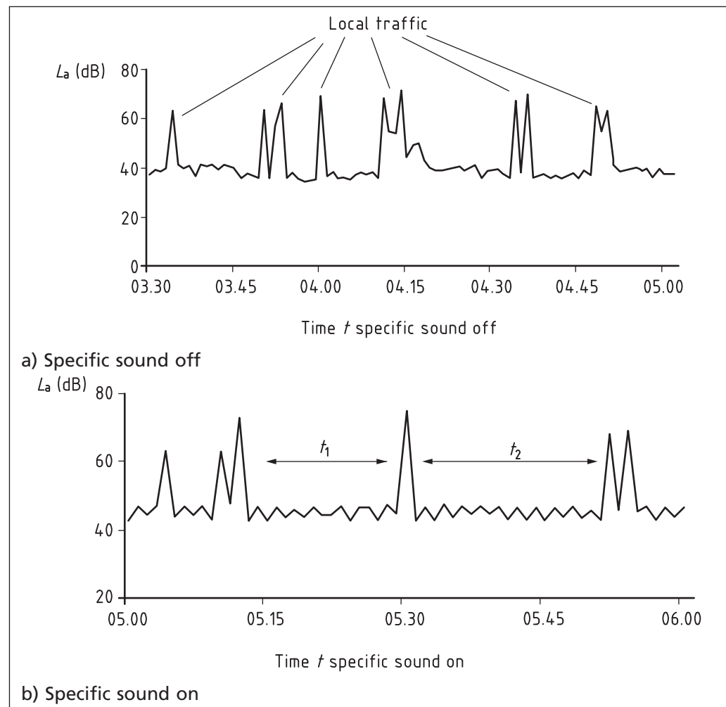
Figure A.3 Sound level variations with time
