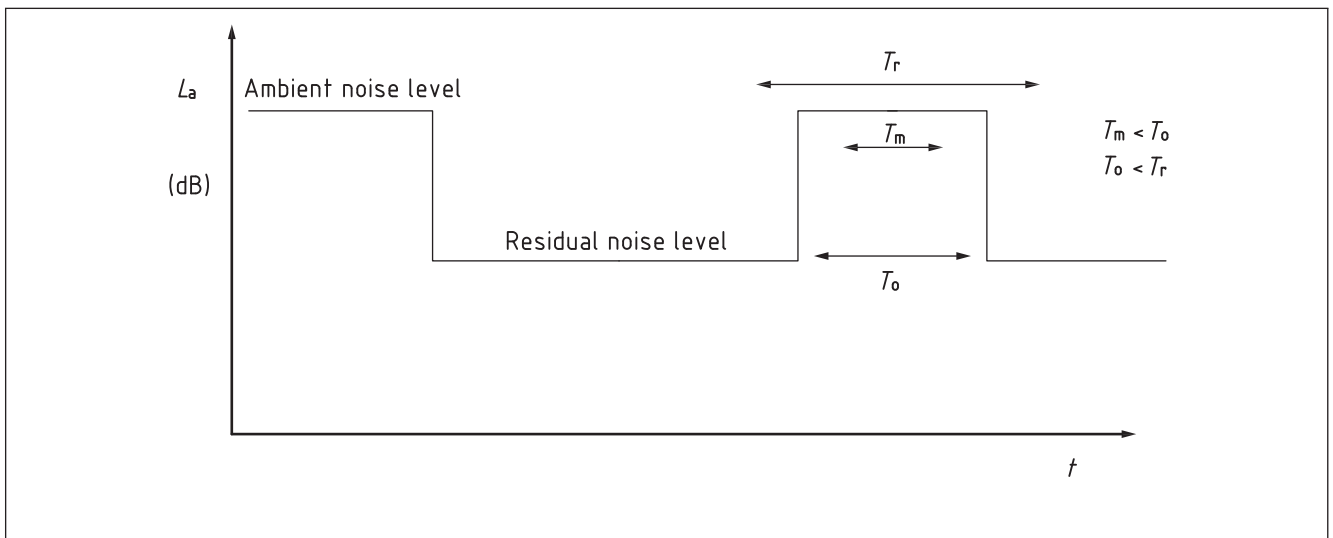
Figure 2 Selecting the measurement time interval
