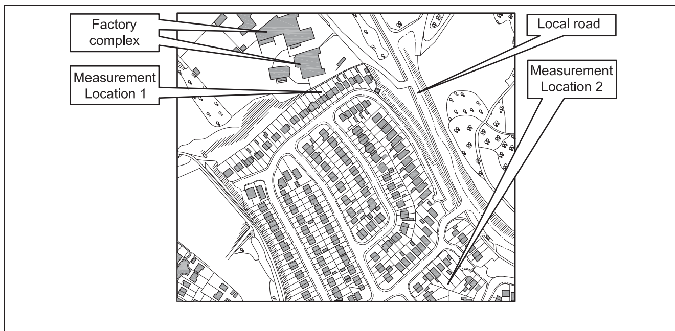
Figure A.9 Measurement locations
